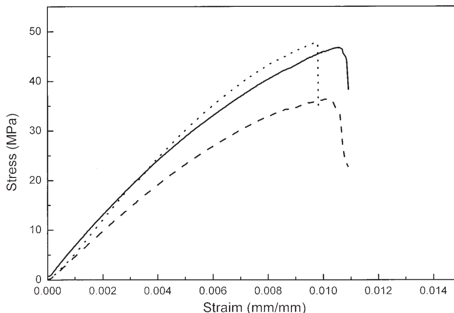
Figure 3 Tensile stress-strain curves for the detergent-washed composites: ( \cdots ) 0, (—) 30, and (---) 45°.
