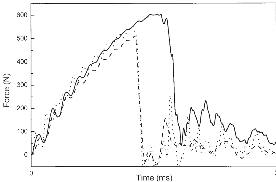
Figure 5 Impact curves (force vs time) obtained from the dry composites: ( — ) as received, ( - - - ) acetone-washed, and ( \cdots ) detergent-washed.
