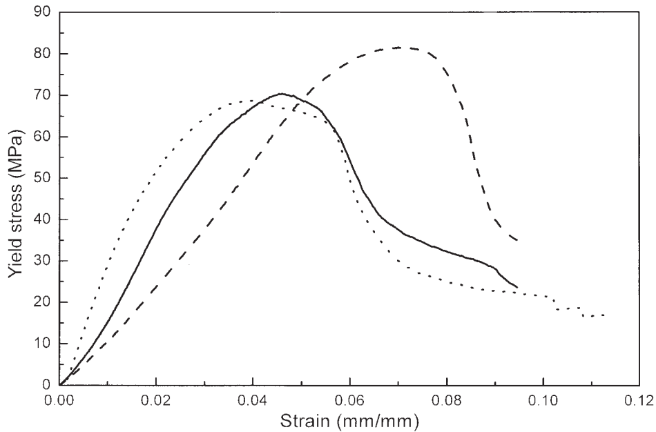
Figure 4 Compressive stress-strain curves for the acetone-washed composites: ( \cdots ) 0, ( — ) 30, and ( - - - ) 45°.
